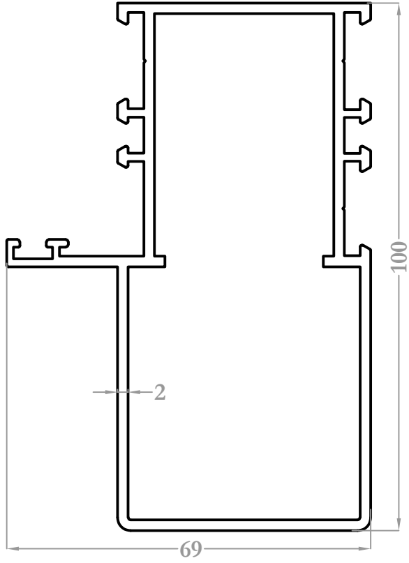
4531 1,929 kg/m
