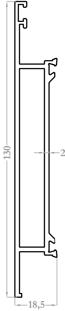
8701 1,393 kg/m
