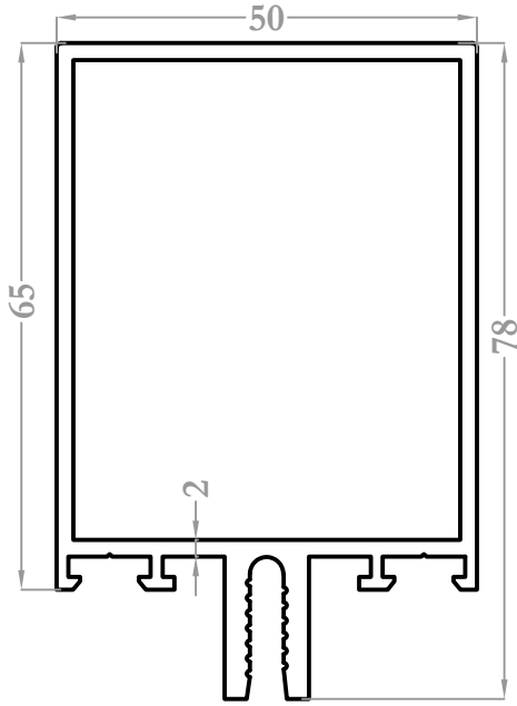
3215 1,514 kg/m
