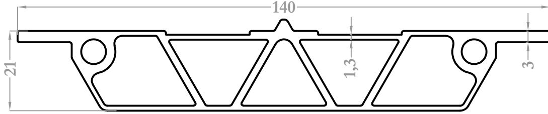
9540 1,941 kg/m
