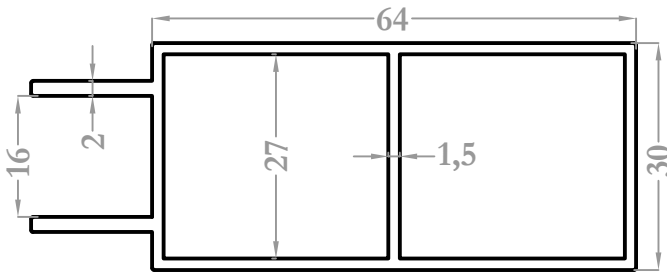
9228 1,023 kg/m
