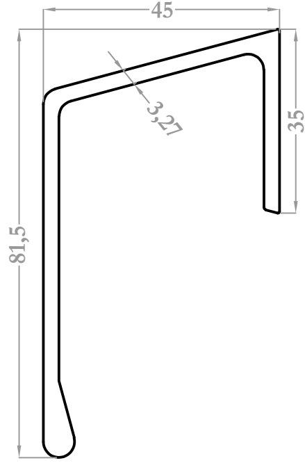
9616 1,248 kg/m
