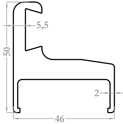
9566 1,817 kg/m
