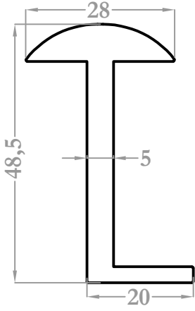
9569 1,068 kg/m
