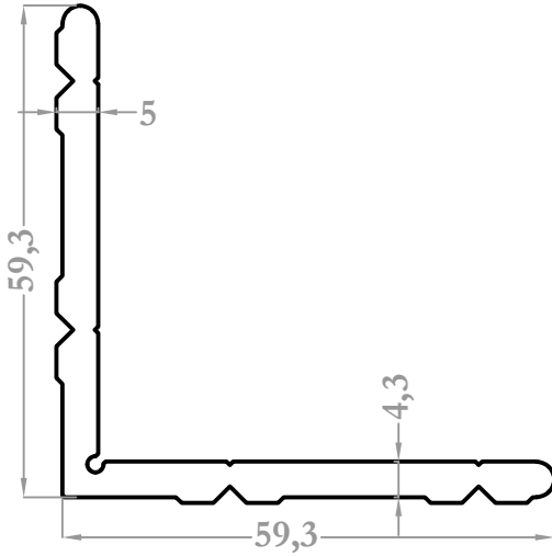
9168 1,362 kg/m
