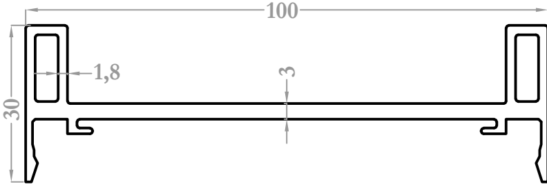
8686 1,303 kg/m
