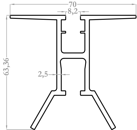
9527 1,411 kg/m
