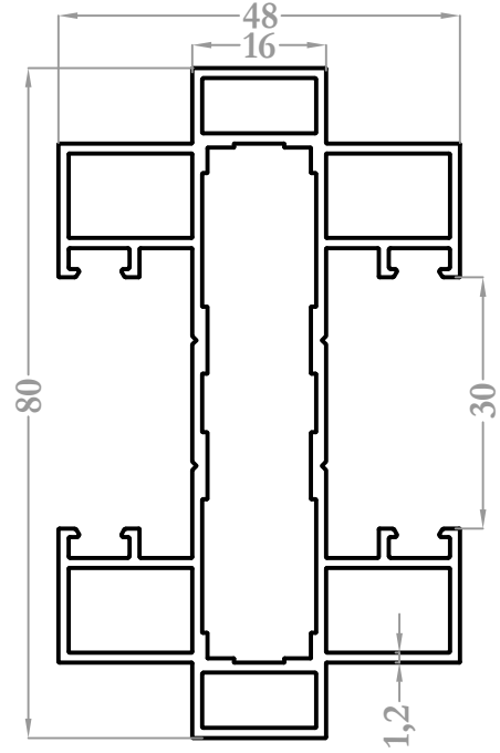
9387 1,447 kg/m
