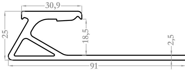
9617 1,262 kg/m
