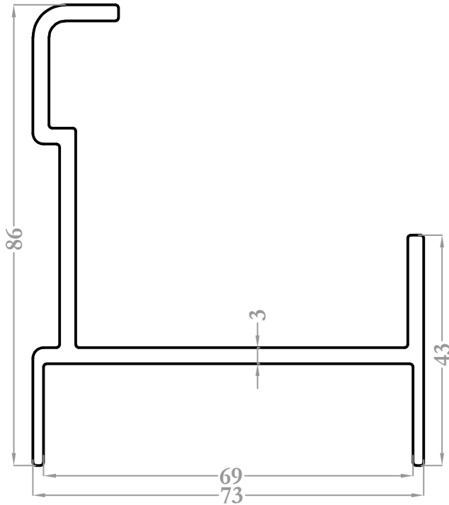
9646 1,616 kg/m
