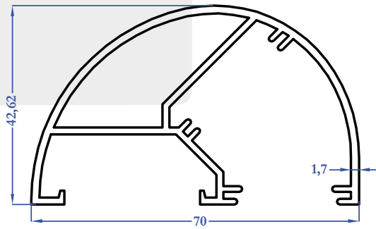
8780 1,000 kg/m
