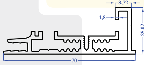
9212 1,029 kg/m
