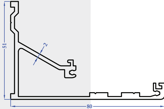
8892 1,046 kg/m
