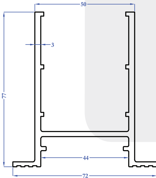
R9099 1,759 kg/m
