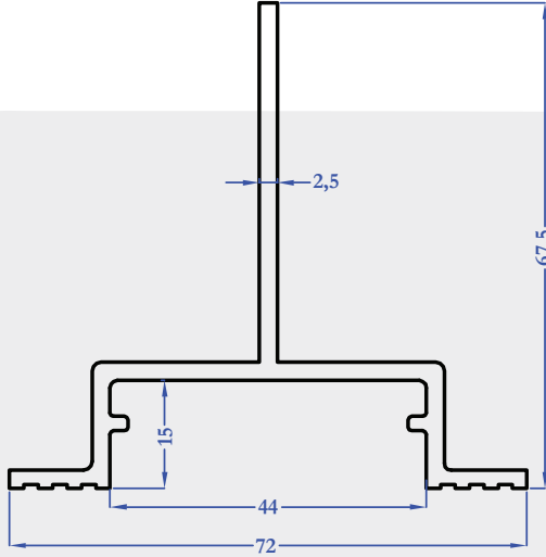
R9031 1,042 kg/m
