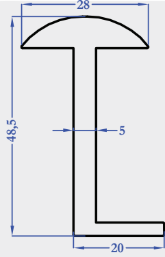
9569 1,068 kg/m
