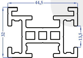
8720 1,322 kg/m
