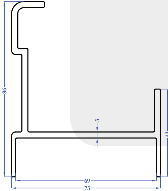
9646 1,616 kg/m
