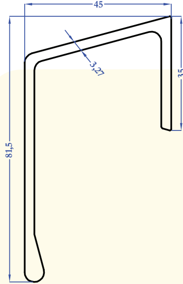
9616 1,248 kg/m
