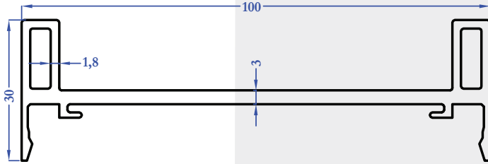
8686 1,303 kg/m
