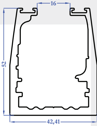
9016 1,544 kg/m
