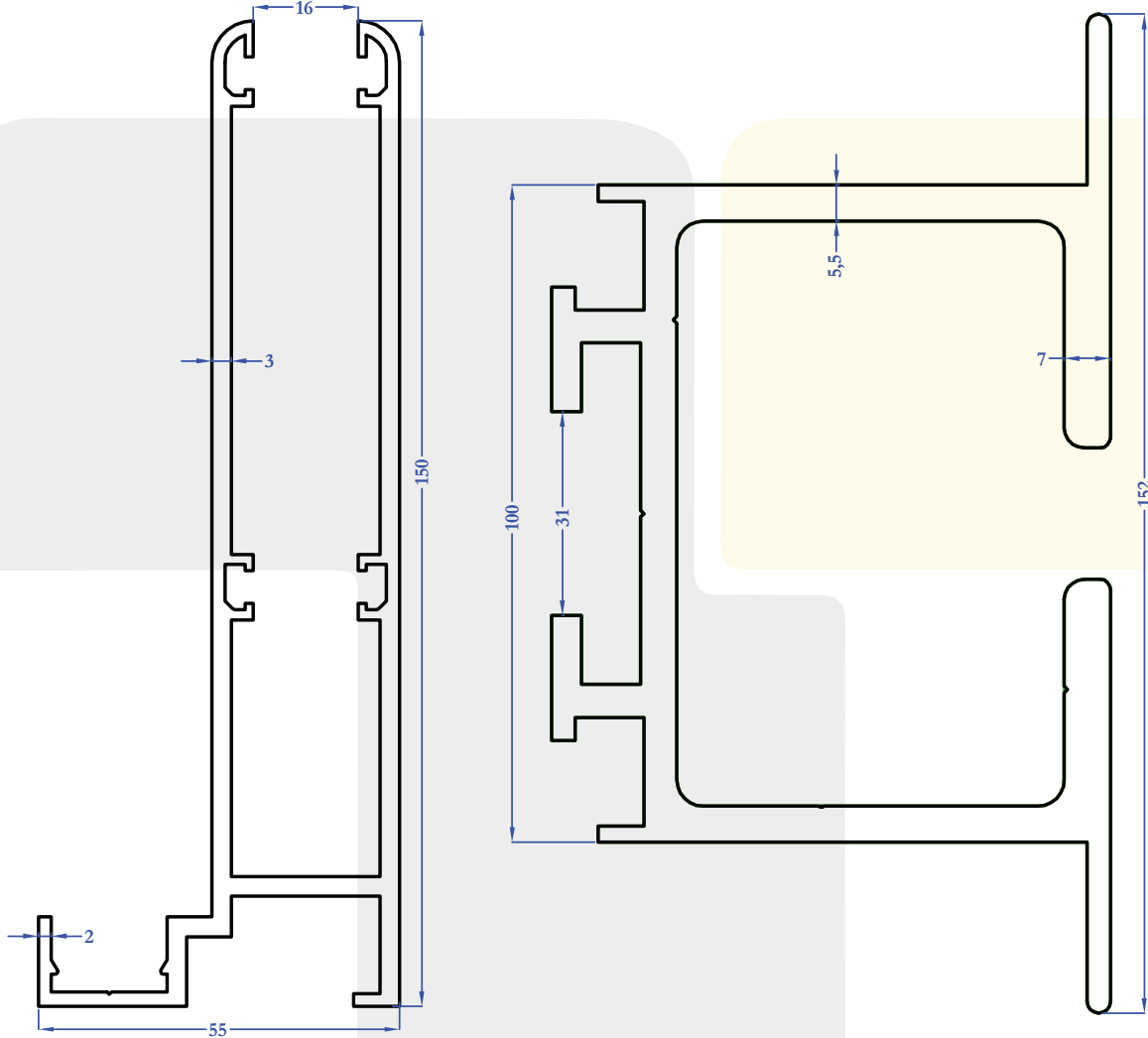
8765 2,940 kg/m
