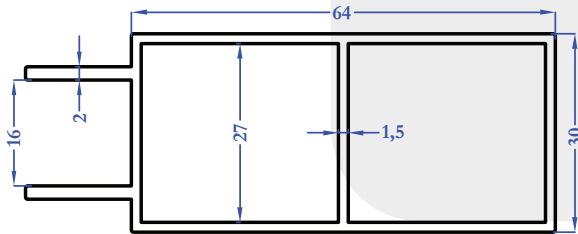
9228 1,023 kg/m
