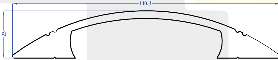
8612 2,560 kg/m
