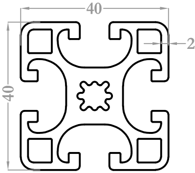
9054 1,763 kg/m
