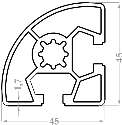
9056 1,462 kg/m
