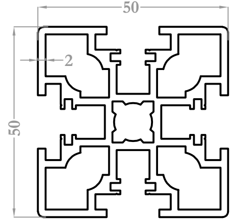
9303 2,118 kg/m
