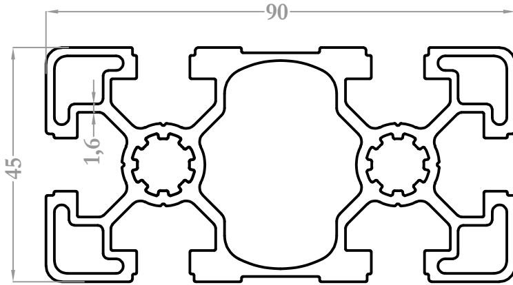
9349 2,943 kg/m
