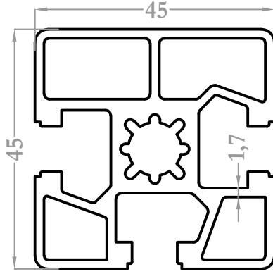
9051 1,766 kg/m
