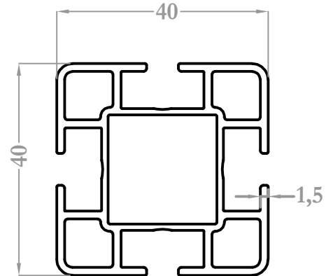
12321 1,023 kg/m
