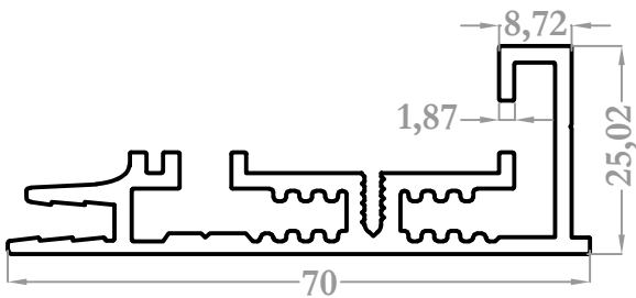
9212 1,029 kg/m
