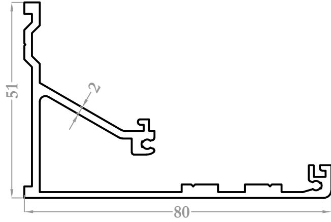
8892 1,046 kg/m
