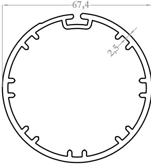
28037 1,625 kg/m
