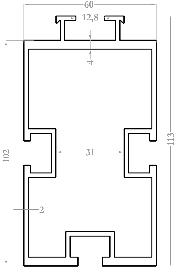
9575 3,009 kg/m
