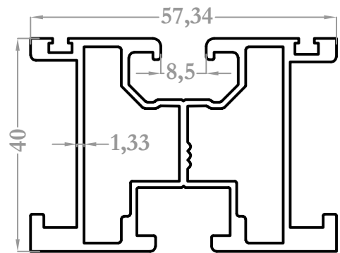
5030 1,362 kg/m
