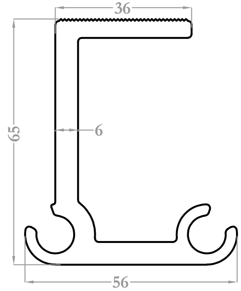
9193 2,260 kg/m
