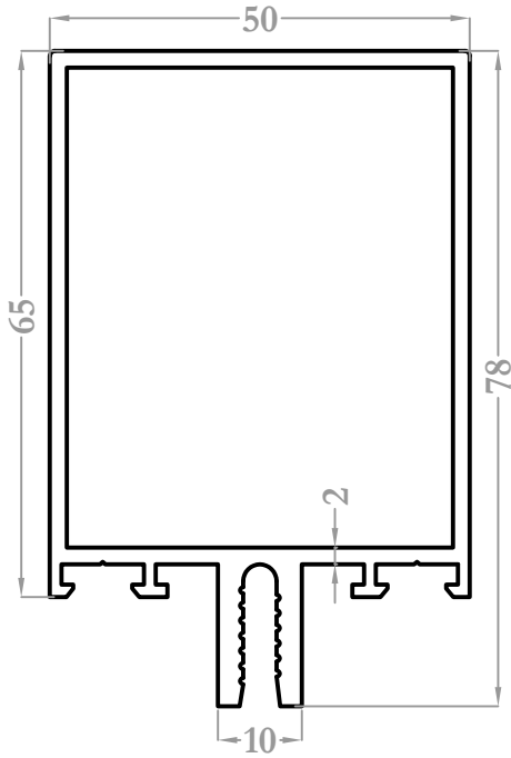
3215 1,514 kg/m
