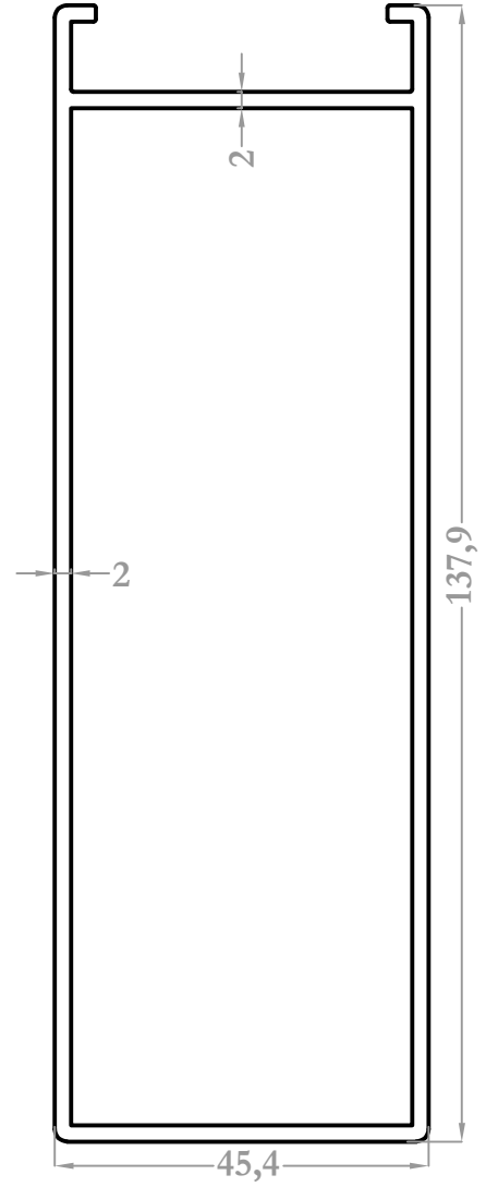
8605 1,970 kg/m
