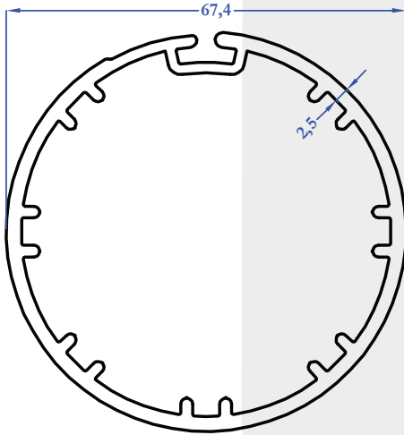
M6008 1,625 kg/m
