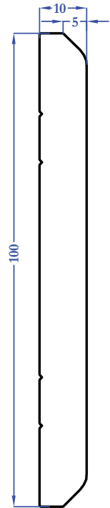
M5134 2,646 kg/m
