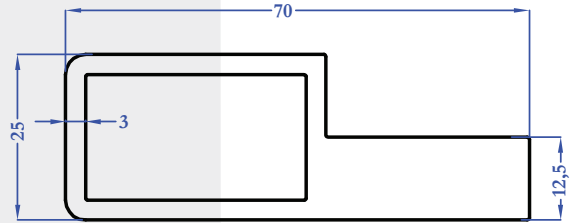
M5391 1,978 kg/m
