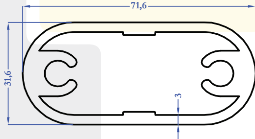
M5150 2,044 kg/m
