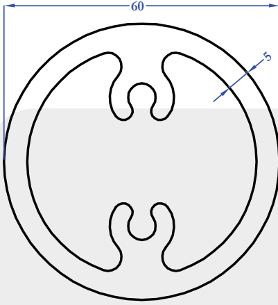
R9040 3,138 kg/m
