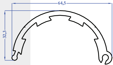
M5506 1,086 kg/m
