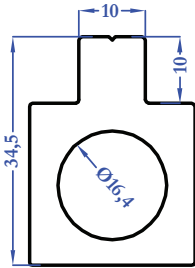
R9045 1,357 kg/m
