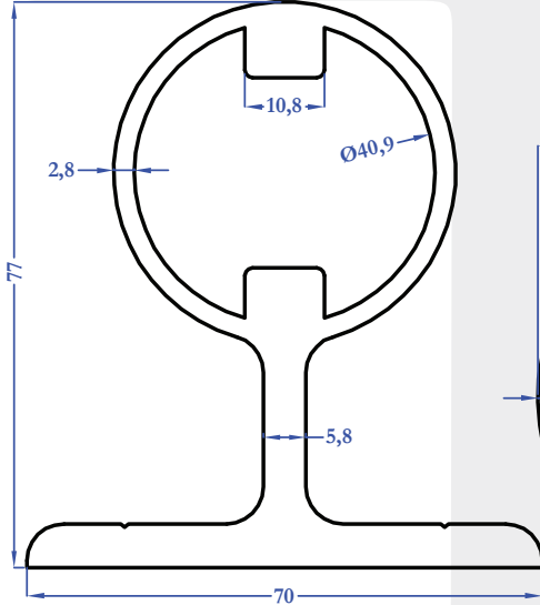
R9235 3,060 kg/m
