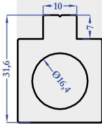
R9066 1,282 kg/m
