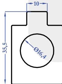
R9065 1.560 kg/m
