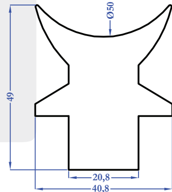
R9046 3,008 kg/m
