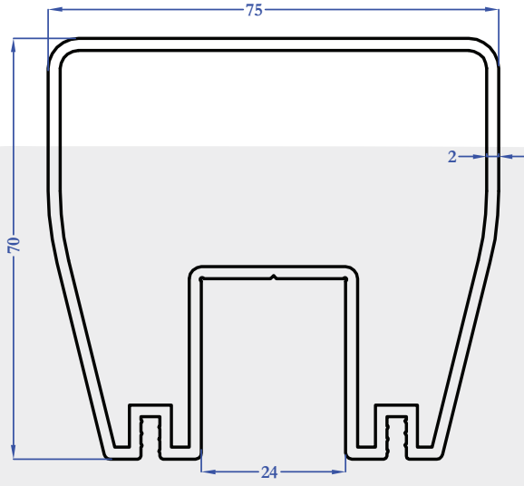
M5057 1,883 kg/m
