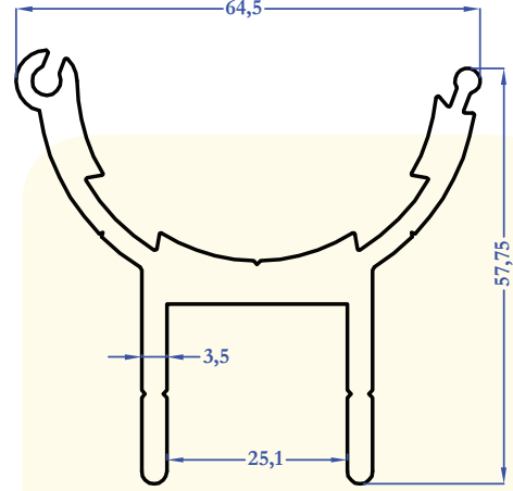
M5507 1,805 kg/m
