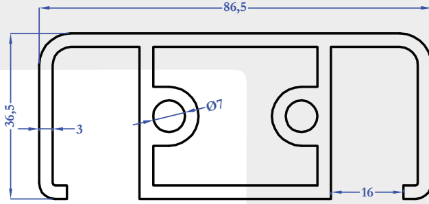
M5153 2,484 kg/m
