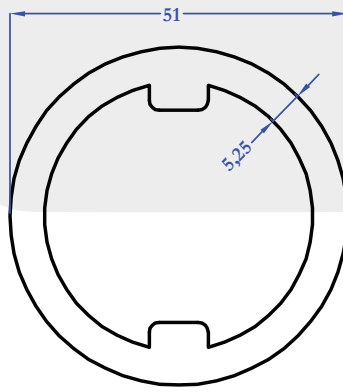
R9042 2,237 kg/m
