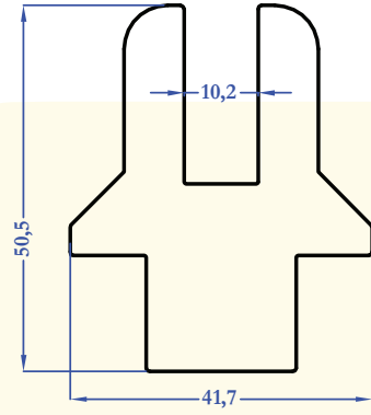
R9048 2,997 kg/m
