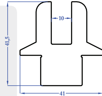
M5108 2,223 kg/m
