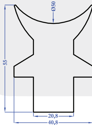
R9049 3,455 kg/m
