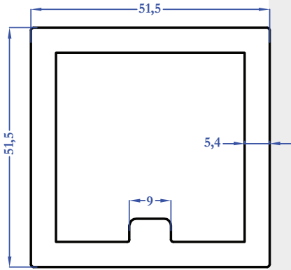
M5392 2,818 kg/m
