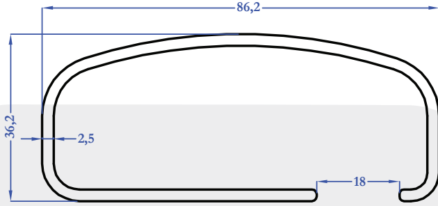
M5044 1,312 kg/m
