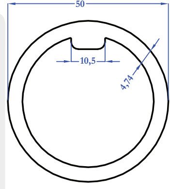
M5113 1,876 kg/m
