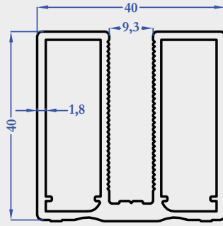
M5455 1,100 kg/m
