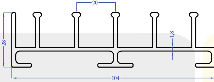
R9136 1,454 kg/m
