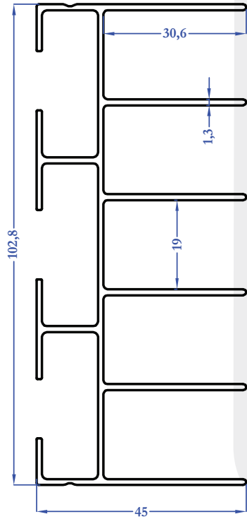
M5246 1,358 kg/m
