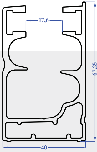
M5005 1,500 kg/m
