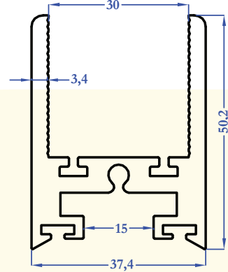
R9004 1,614 kg/m
