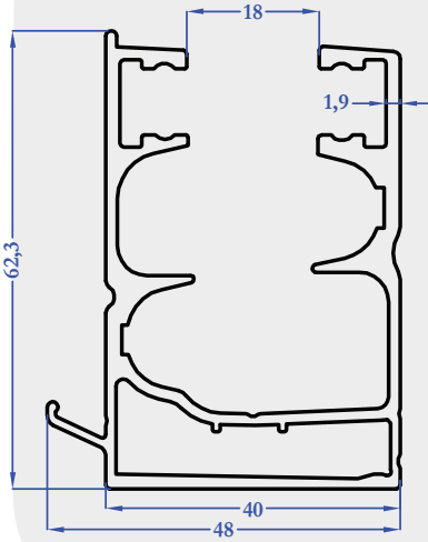
M5683 1,373 kg/m
