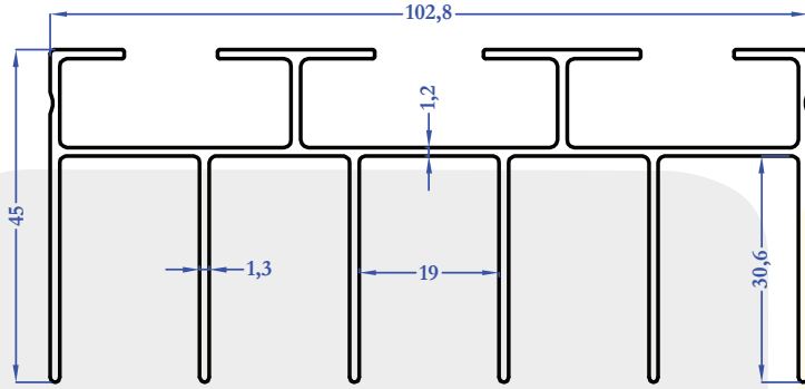
M5246 1,358 kg/m
