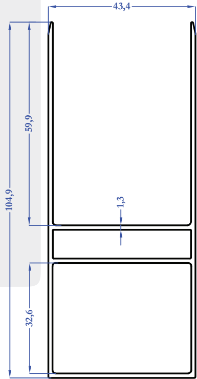
M5686 1,150 kg/m
