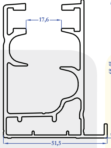
M5196 1,545 kg/m
