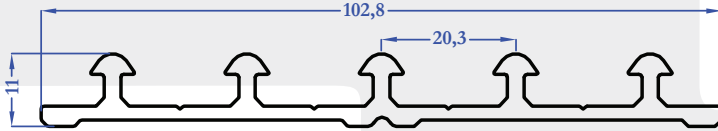
M5247 1,010 kg/m
