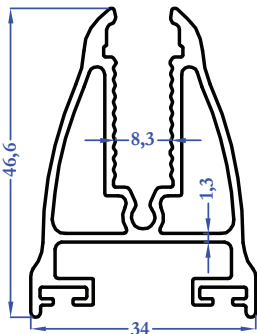
M5004 0,882 kg/m
