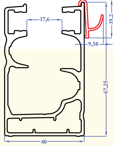
M5689 1,428 kg/m
