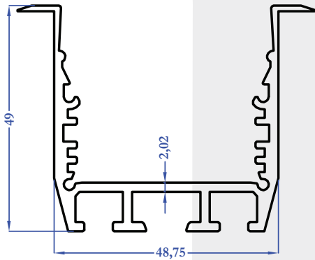
9507 1,129 kg/m
